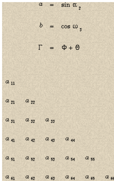
Figure 12: How math2html translates \text{\LaTeX} multi-line mathematics into HTML3
